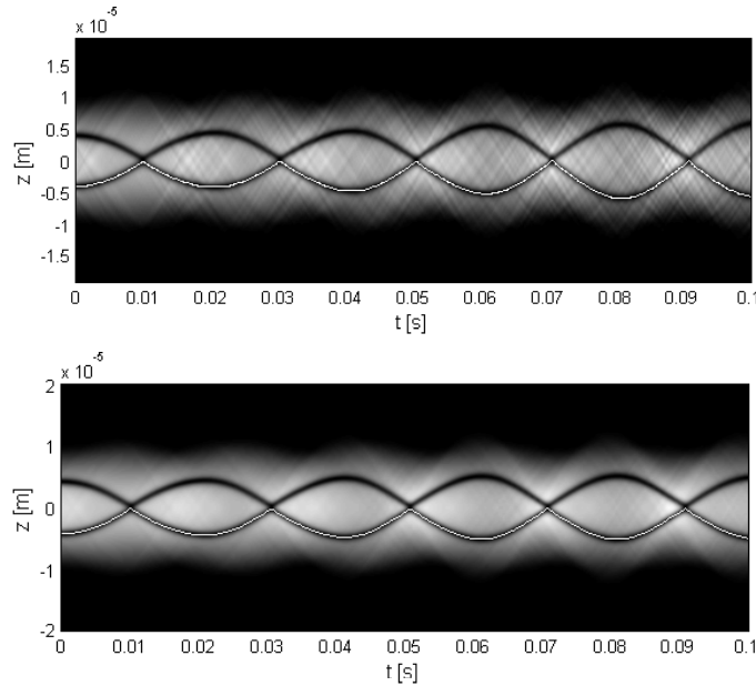
Figure 2.14: top: Two soliton IS simulation using the 3D GPE resulting in \nu_d = 0.744 . bottom: Two soliton IS simulation using the NPSE resulting in \nu_d = 0.751 . The path of the density minimum of one of the solitons is shown by the white lines. For the parameter sets of our measurements (see section 4.2) we checked the difference of the oscillation frequency obtained by numerical simulations using the NPSE from the 3D GPE result. For the mean deviation of \nu_{3DGPE} - \nu_{NPSE} we get \Delta(\nu_{3DGPE} - \nu_{NPSE}) = 1\% \pm 0.6\% . Parameters: Set #4 of tables 4.1 and 4.2.
