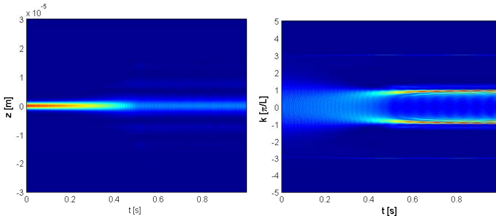
Figure A.1: Numerical simulation using the MDE of the creation of a bright soliton by the method of Matuszewski et al.. left: Time evolution of the atomic density in real space. At t = 0.5 \text{ s} the soliton has been created. right: Time evolution of the atomic density in momentum space. The momenta accumulate at the edges of the first Brillouin zone at k = \pi/L . Parameters: See text
