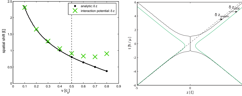
Figure 2.10: left: Analytically calculated spatial shifts and comparison with the shifts of the soliton trajectories obtained from the interaction potential approach. Symmetric case: \nu = \nu_1 = -\nu_2 . The velocity \nu = 0.5 is marked by the dashed line. We see that for \nu < 0.5 both approaches agree very well. In the regime \nu \geq 0.5 the interaction potential cannot be applied. right: Illustration of the difference between the shift obtained from analytic calculation \delta z_{analytic} and from the interaction potential \delta z_{ODE} .
