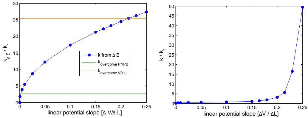
Figure A.8: left: Possible momenta which the soliton can gain from a linear potential slope, otherwise similar to Fig. A.5(left). right: Effectively gained momenta of the atom cloud. Similarly to the case of a harmonic slope the atoms start leaking out of the lattice sites for \Delta V / L \gtrsim V_0 - \mu . In this case the soliton is destroyed and the atom cloud can gain a high overall momentum down the slope.
