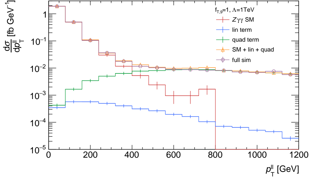
Figure H.1.: Validation of the decomposition approach for the differential p_T^{\ell\ell} cross section predicted by \mathcal{O}_{T,9}^8 with f_{T,9} = 1 and \Lambda = 1 TeV in the fiducial phase-space. The orange distribution contains the sum of the SM (red), linear term (blue), and quadratic term (green). The full simulation (magenta) contains the predicted differential cross section when generating the full SM plus EFT amplitude.
