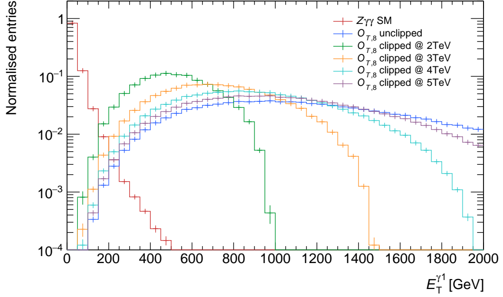
Figure 8.5.: Effect of clipping procedure on E_T^{\gamma 1} predicted by \mathcal{O}_{T,8}^8 (quadratic term only) for E_c thresholds between 2 and 5 TeV. The distribution of the SM expectation, which is not truncated, is shown as reference.
