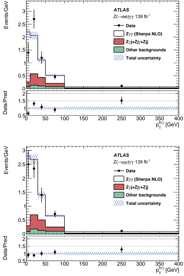
Figure E.2.: The observed p_T^{\ell\ell\gamma\gamma} distribution is shown in (a) the electron channel and (b) the muon channel. It is compared to the sum of the total background contribution and the Z\gamma\gamma prediction. The uncertainty band accounts for the statistical and systematic uncertainties on the number of background events, and for the CP uncertainties of the signal process. The figures are taken from [41].
