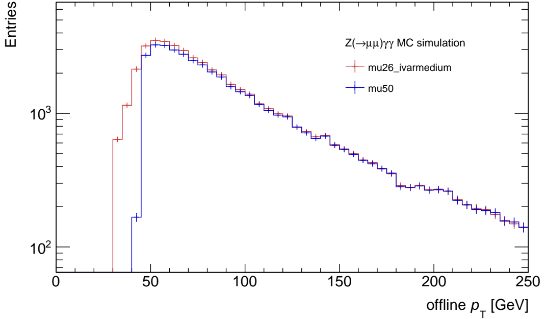
Figure 5.5.: In all simulated Z(\rightarrow\mu\mu)\gamma\gamma events surviving the event selection, it is tested which of the single muon trigger items listed in Table 5.2 have been fired as a function of the p_T of the leading offline muon. Trigger items that were only active in 2015 are omitted.
