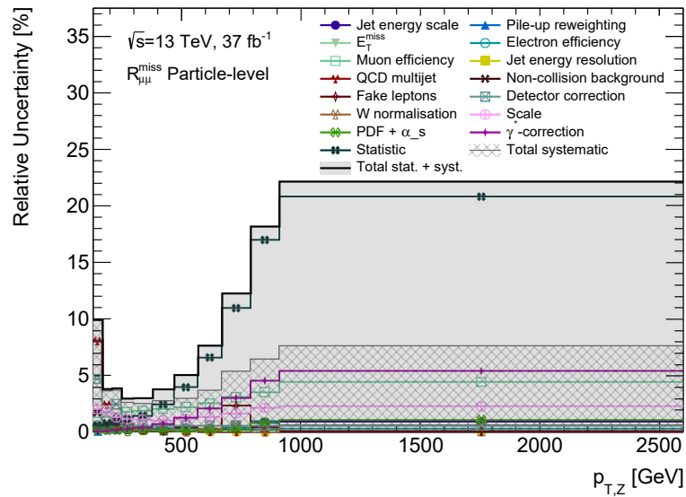
Figure 10.5: Relative uncertainties on the R_{ee}^{\text{miss}} (top) and R_{\mu\mu}^{\text{miss}} (bottom) ratio at particle level. Only systematic uncertainties with a contribution of at least 0.5% in any bin are presented. The shown uncertainties are symmetrized.
